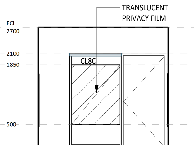
2 ELEVATION DETAIL 1 : 50
