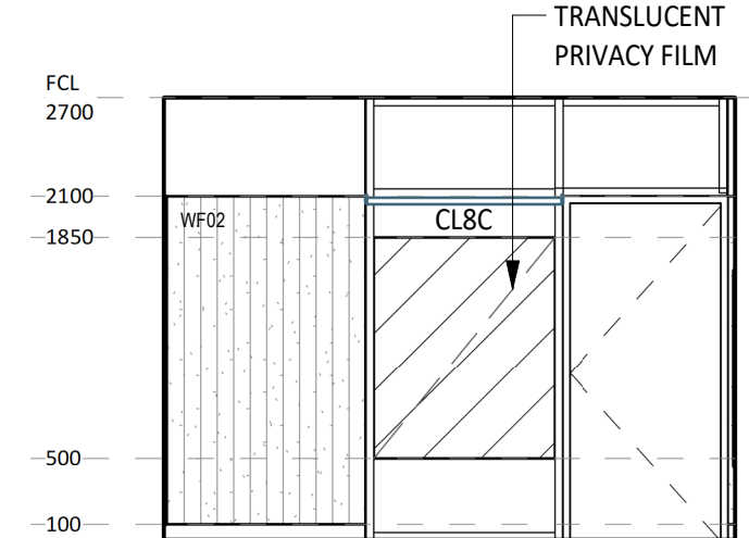
11 ELEVATION DETAIL 1 : 50
