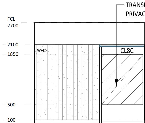
8 ELEVATION DETAIL 1 : 50
