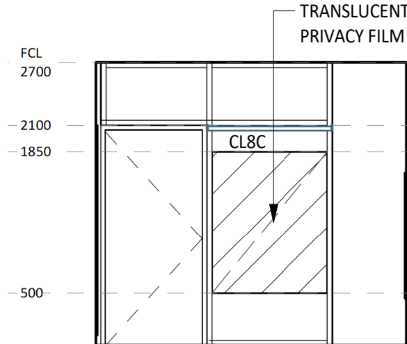
7 ELEVATION DETAIL 1 : 50
